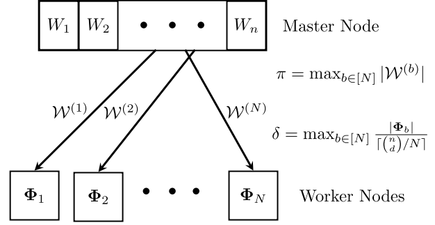
Fig. 1. Distributed computing model. The set of files communicated to worker b is denoted with \mathcal{W}^{(b)} = \alpha(\Phi_b) , while \pi denotes the maximum communication cost across the master-worker links under the assumption of parallel, uniform-capacity links. Similarly, the set of subfunctions assigned for computation to worker b is denoted by \Phi_b , while \delta denotes the computational delay normalized by the minimum possible computational delay, assuming homogeneous workers.
