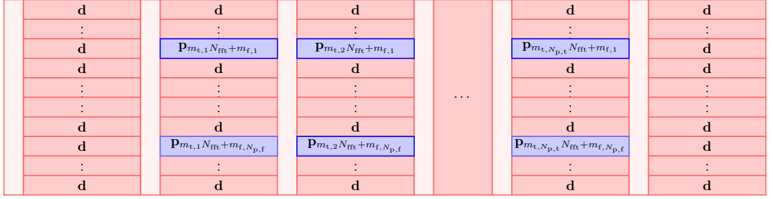
Figure 2.3: OFDM frame with pilot (blue), guard (light blue and red) and data (red) subcarriers. Each symbol is preceded by L - 1 CP samples (light red)
