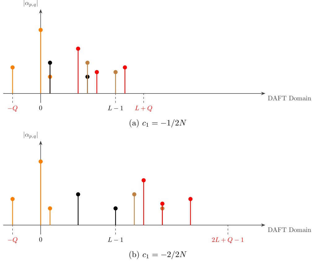
Figure 2.6: DAFT domain representation of the channel realization of Figure 2.1b for different values of c_1
