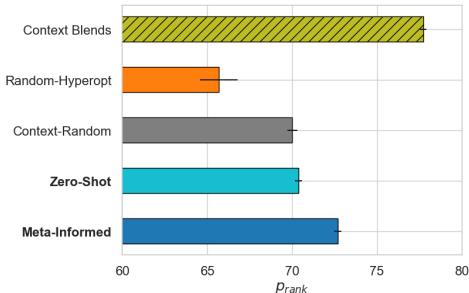
Figure 2: Comparison of prompting strategies and baselines in terms of p_{\text{rank}} . The Context Blends produced by AutoML performance for each challenge are shown as a reference. Error bars indicate 90% confidence intervals of the mean across 8 random seeds per dataset.
