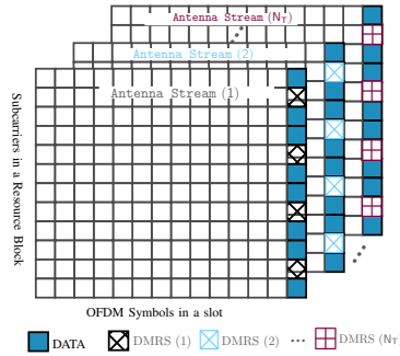
Figure 4.2: Conceptual illustration of DMRS density per stream in MIMO Configuration
