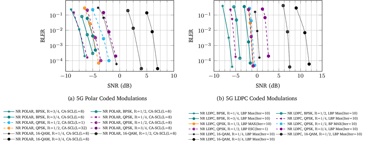
Figure 2.12: Block Error Rate, 100 bits(TBs+CRC), R=\{1/4, 1/2, 3/4\} , NR LDPC (BP, LBP with Early Stop Criteria (ESC), MaxIter=10) and NR POLAR, (CA-SCL, L=1, 8, 32 ), {BSPK, QPSK, 16-QAM modulations}, over (1 \times N_R = 4) SIMO, on TDL (NLOS channel, 300ns of delay spread).
