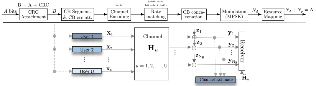
Figure 4.3: Conceptual Illustration of K – users within: (N_R \times N_T) MAC MIMO system in a block fading environment
