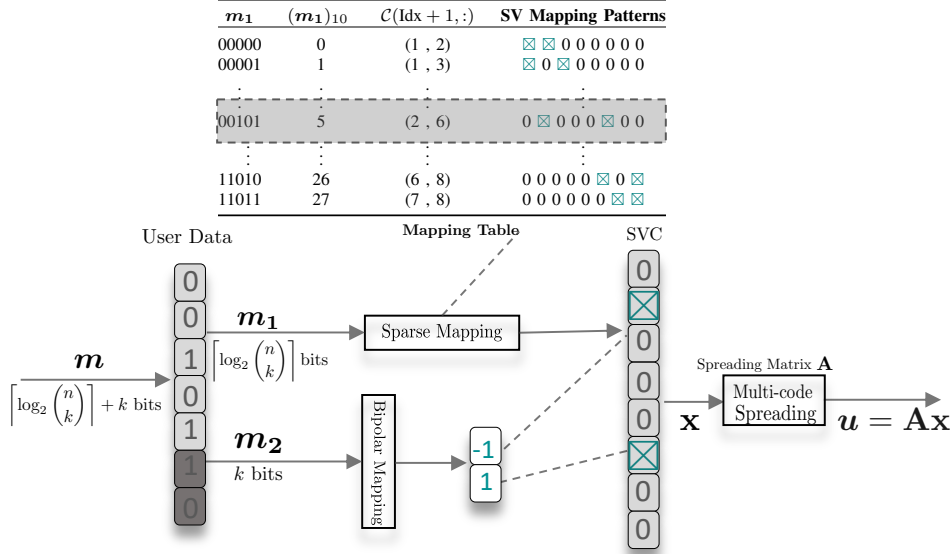
Figure 5.6: Conceptual illustration of Sparse Vector Coding ( n = 8, k = 2 ): Encoder side.
