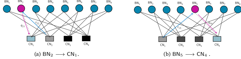
Figure 2.5: Bit Node Updates
