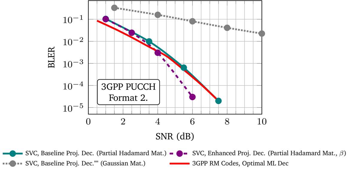
Figure 5.11: Block Error Rate, 3GPP PUCCH 2 : {1 OFDM symbol, 4 PRBs, 32 Data REs, 16 DMRS REs}, Sparse Vector Coding : {sparse vector length n = 32 , sparsity level k = 2 , message m = 11 bits SV Coding Rate = 11/32 }, 3GPP Reed Muller Coding \mathcal{C}(32, 11) : {message m = 11 , RM Coding Rate = 11/32 , QPSK modulation}, Decoders : {Baseline partial Hadamard matrix projection decoding vs LLR-based attention-weighted Hadamard matrix projection decoding vs Maximum likelihood decoding for 3GPP RM codes}, Channel Configurations : { Unknown CSI transmission, Least Squares channel estimation + linear Interpolation, (1 \times N_R = 4) 3GPP TDL-C NLOS (Long Delay Spread = 300 ns, Sampling rate f_s = 30.72 MHz) channel. }
