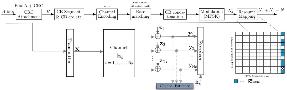
Figure 3.1: Bit-Interleaved Polar/LDPC coded Modulation (BIPCM/BILPCM) : Transmitter end.
