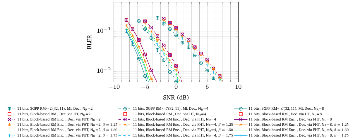
Figure 5.4: Block Error Rate, 11 bits, 2 PRB(16 REs=data, 8 REs=DMRS), Block-based decoding via HT & FHT based decoders vs ML decoder, adaptive DMRS/data power adjustment bia \beta , (\{8, 4, 2\} \times 1) SIMO, Rayleigh fading Channel, Unknown Channel State Information.
