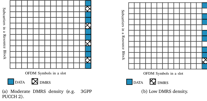
Figure 3.2: General resource mapping: 1 OFDM symbol.
