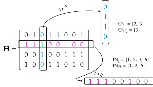
Figure 2.6: Conceptual Illustration of CNs and BNs processing Within BN and CN index sets for the specified values of i and j .
