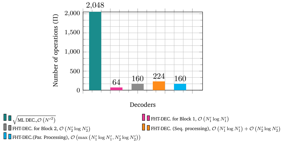
Figure 5.5: Comparative analysis, showing the number of \Pi operations for the ML decoder compared to block-based FHT-decoders featuring sequential and parallel processing.
