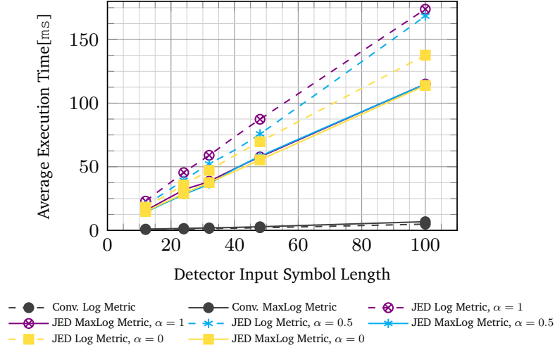
Figure 3.7: Average Time Complexity of the proposed SIMO JED metrics vs Conventional metrics.
