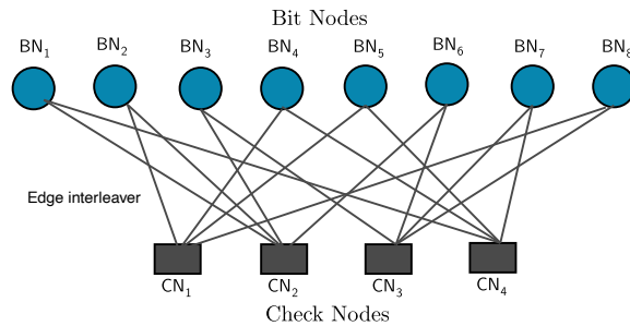
Figure 2.1: Parity check matrix \mathbf{H}(4, 8) and the corresponding Tanner graph
