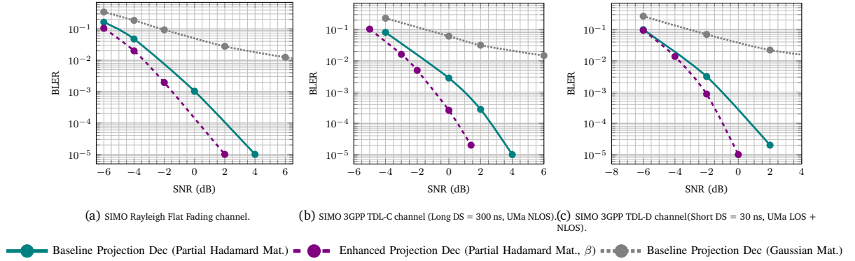
Figure 5.9: Block Error Rate, Sparse Vector Coding : {sparse vector length n = 64 , sparsity level k = 2 , spreading matrix \mathbf{A} \in \mathbb{R}^{m=32 \times n} , message \mathbf{m} = 13 bits ( \mathbf{m} = 11 bits + \mathbf{m}_2 = 2 bits), SV Coding Rate = 13/64 }, Decoders : {Baseline partial Hadamard matrix projection decoding vs Baseline random Gaussian matrix Projection decoding vs LLR-based attention-weighted Hadamard matrix projection decoding }, Channel Configurations : { Perfect Channel State Information transmission, ( 1 \times N_R = 4 ) SIMO Rayleigh flat fading channel, 3GPP TDL-C NLOS (Long Delay Spread = 300 ns), 3GPP TDL-D LOS + NLOS (Short Delay Spread = 30 ns), Sampling rate f_s = 30.72 MHz) channels. }
