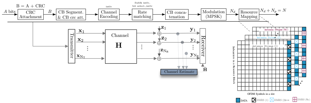
Figure 4.1: Bit-Interleaved Polar/LDPC coded Modulation (BIPCM/BILCM), a (N_T \times N_R) SU-MIMO System.
