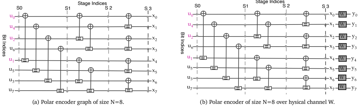
Figure 2.7: The graph of an (8, 4) polar code with bit reversed indexing transmitted over physical channels ( W ).
