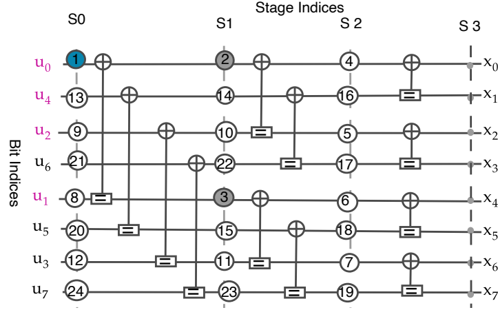
Figure 2.10: Illustrative instance of a recursive order.
