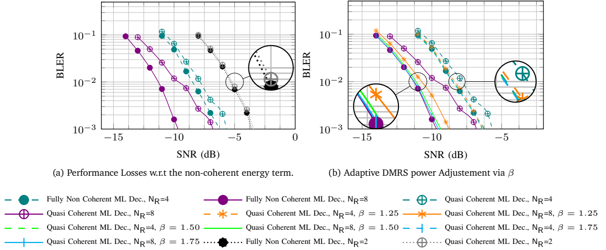
Figure 5.1: Block Error Rate, 4 bits, (SIMO, 3GPP TDL-C urban NLOS channel, 300ns of Delay spread, Unknown Channel State Information)
