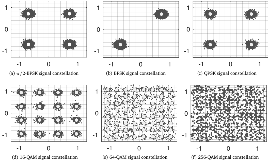
Figure 2.11: Gray Labelling modulation constellation sets at noise-free and SNR=-20 dB.
