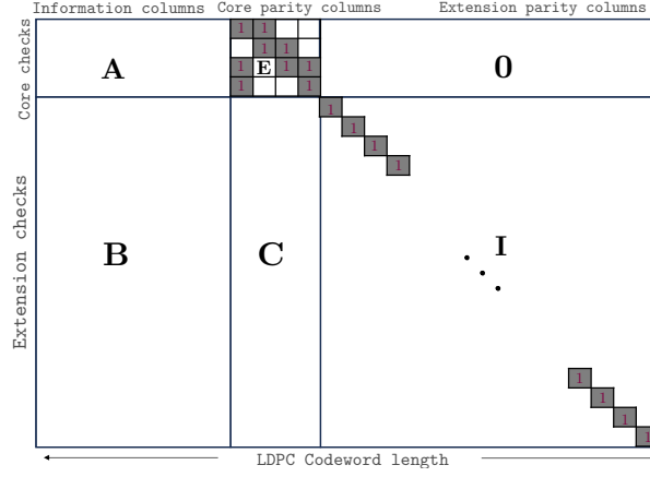
Figure 2.2: 3GPP NR Base graphs structure.
