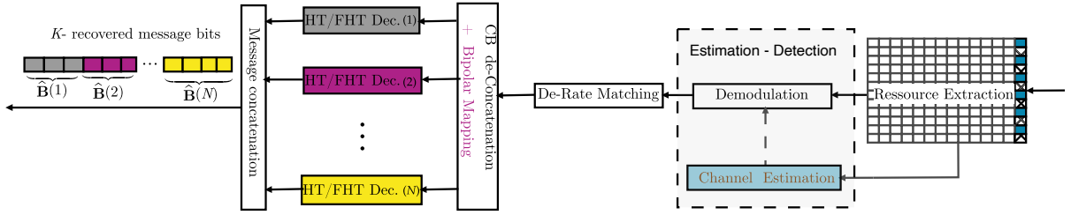
Figure 5.3: Block-based HT/FHT based-decoding of Short blocks : Receiver end.
