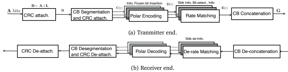
Figure 2.8: Conceptual illustration of 5G Polar transceiver chain.
