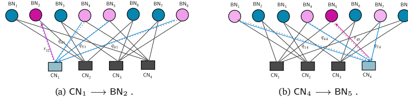
Figure 2.4: Check Node Updates
