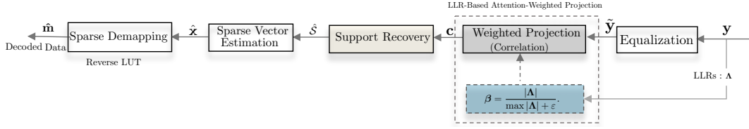
Figure 5.7: Conceptual illustration of the SVC receiver using LLR-based attention-weighted projection decoding.
