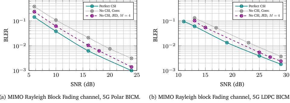
Figure 4.4: Block Error Rate, 48 bits(TBs+CRC), NR POLAR BICM (CRC-aided successive-cancellation list decoder, List length=8), NR LDPC BICM (belief propagation decoder, iteration=30) QPSK modulation, 1 OFDM symbol, 4 PRBs, 48 REs (32 data, 16 DMRS), (4 \times 4) MIMO.
