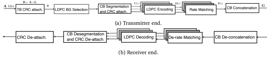
Figure 2.3: Conceptual illustration of 5G LDPC transceiver chain.
