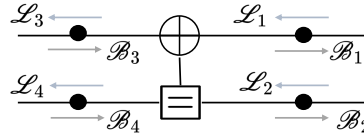
Figure 2.9: Factor Graph of the SC decoding unit.
