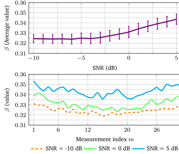
Figure 5.10: Average \beta values as a function of SNR and the \{\beta_i\}_{i=1}^m values over different SNRs, Sparse Vector Coding : \{n = 64, k = 2, \mathbf{A} \in \mathbb{R}^{m=32 \times n}\} , 3GPP TDL-C NLOS (Long Delay Spread = 300 ns) channels.
