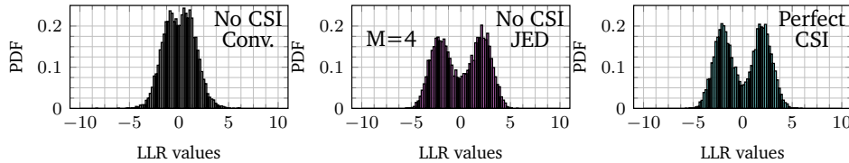
Figure 3.6: LLR distribution characteristics via histograms at SNR = 0 dB.
