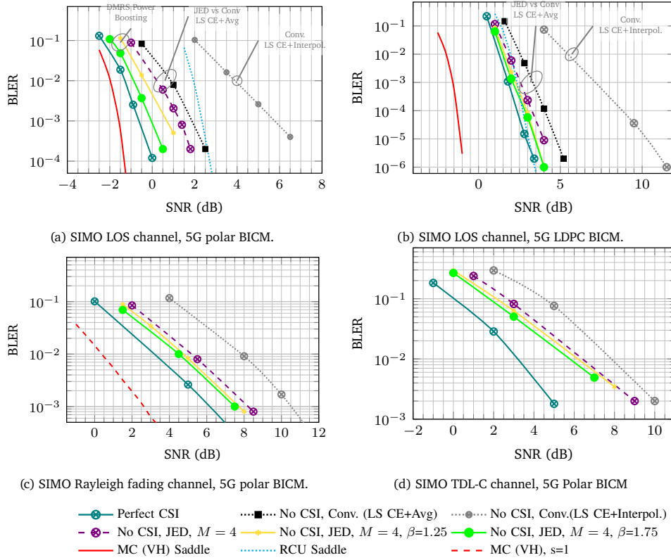
Figure 3.5: Block Error Rate, 48 bits(TBs+CRC), NR POLAR BICM (CRC-aided successive-cancellation list decoder, List length=8), NR LDPC BICM (belief propagation decoder, iteration=30) QPSK modulation, 1 OFDM symbol, 4 PRBs, 48 REs (32 data, 4 DMRS), (1 \times 4) SIMO, vs outer (MC) and inner (RCUs) bounds, DMRS power Boosting via a scaling factor \beta .
