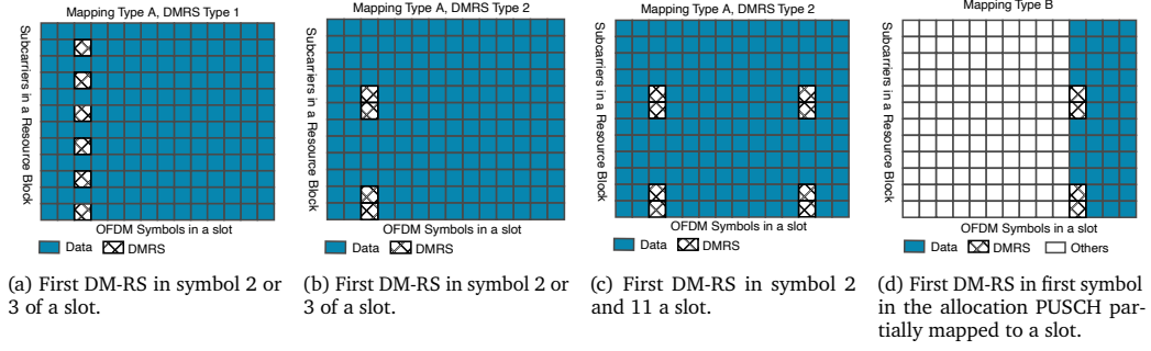
Figure 3.3: DMRS PUSCH based resource mapping for JED oriented receiver.
