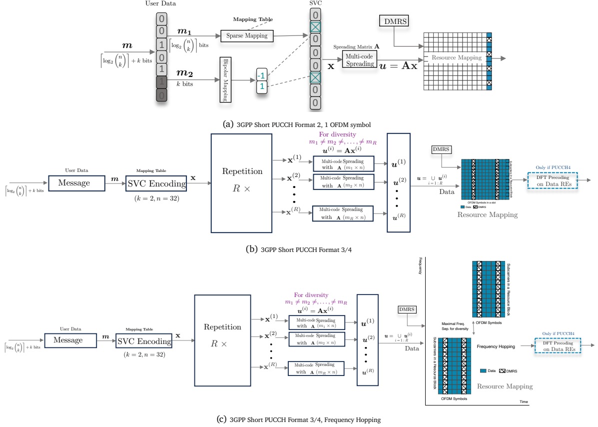
Figure 5.8: Conceptual illustration of sparse vector coded transmission for 3GPP PUCCH (e.g., Formats 2, 3 &amp; 4).
