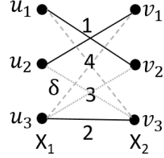
Fig. 1. Bipartite graph for Example 1 where the function outcomes are indicated on the edges, the bipartite vertex sets denote the outcomes X_1 and X_2 , respectively, and each dotted or dashed edge has a probability \delta .
